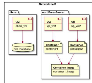
Figure 1. First DOML example in PIACERE project illustrates how realistic applications and their supporting infrastructure can be specified
